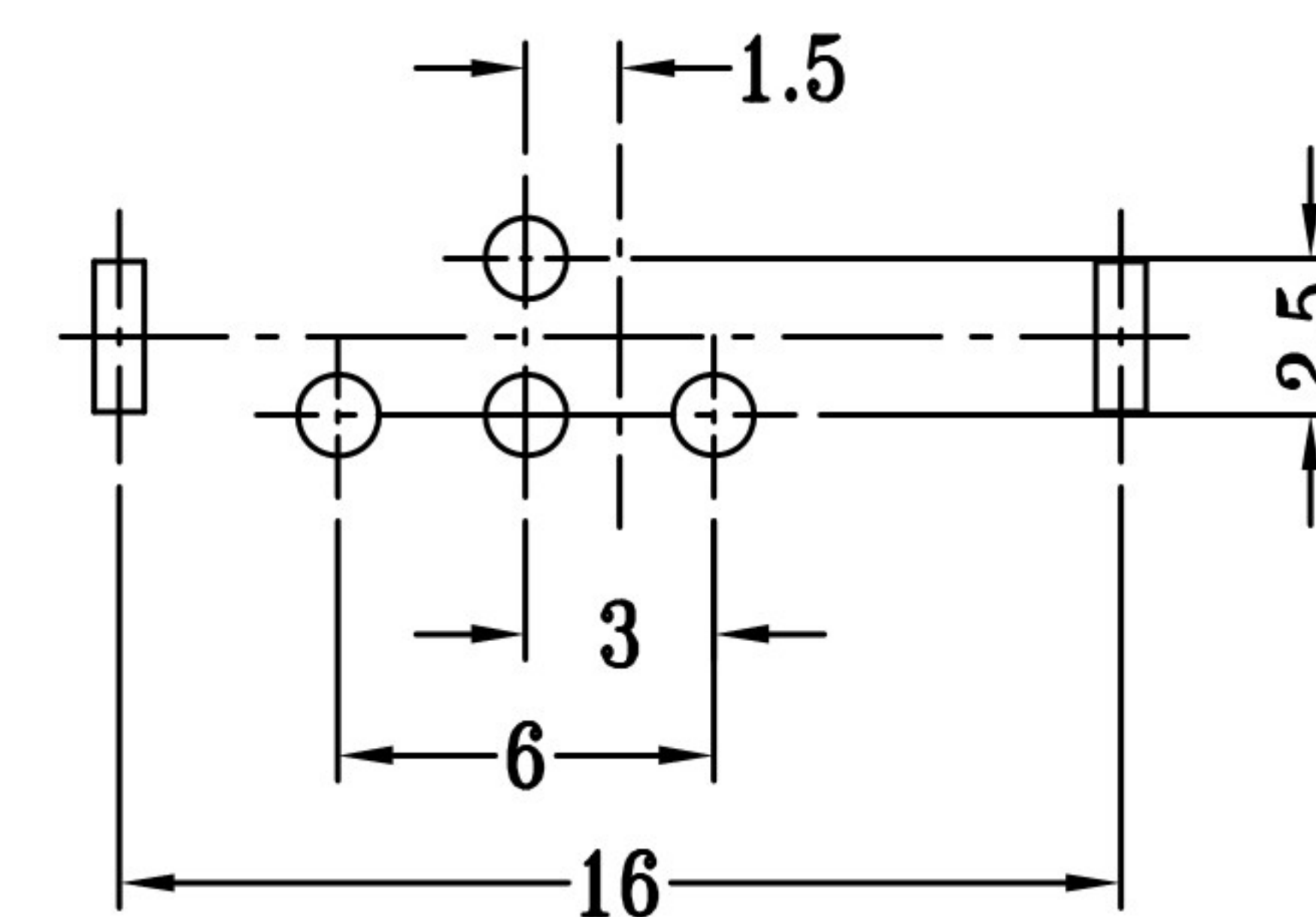
P.C.B LAYOUT BOTTOM VIEW
