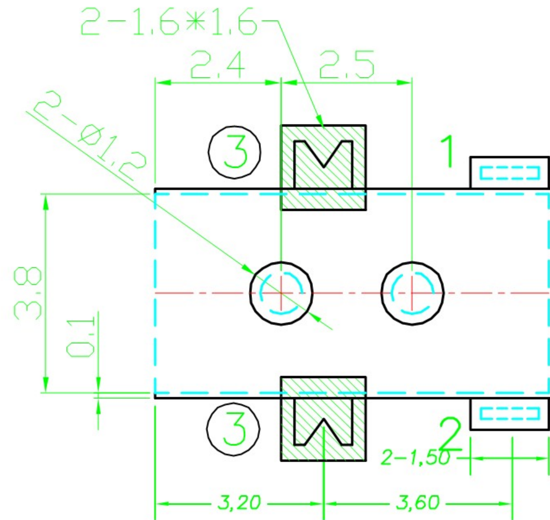
P.C.B LAYOUT TOP VIEW
