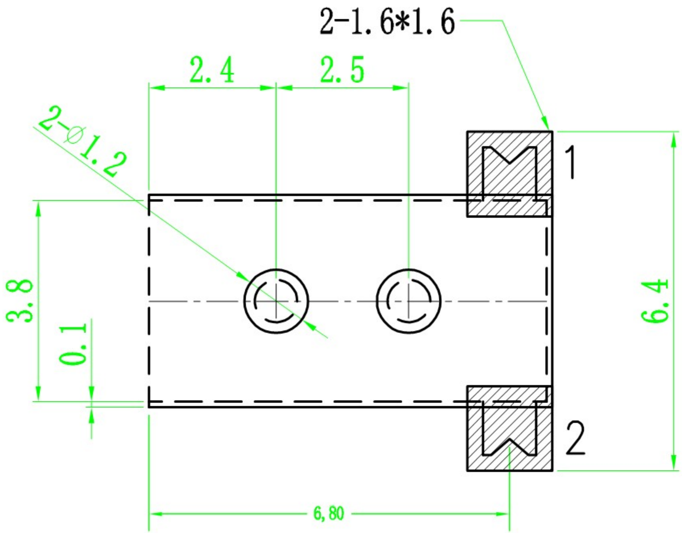
P.C.B LAYOUT TOP VIEW
