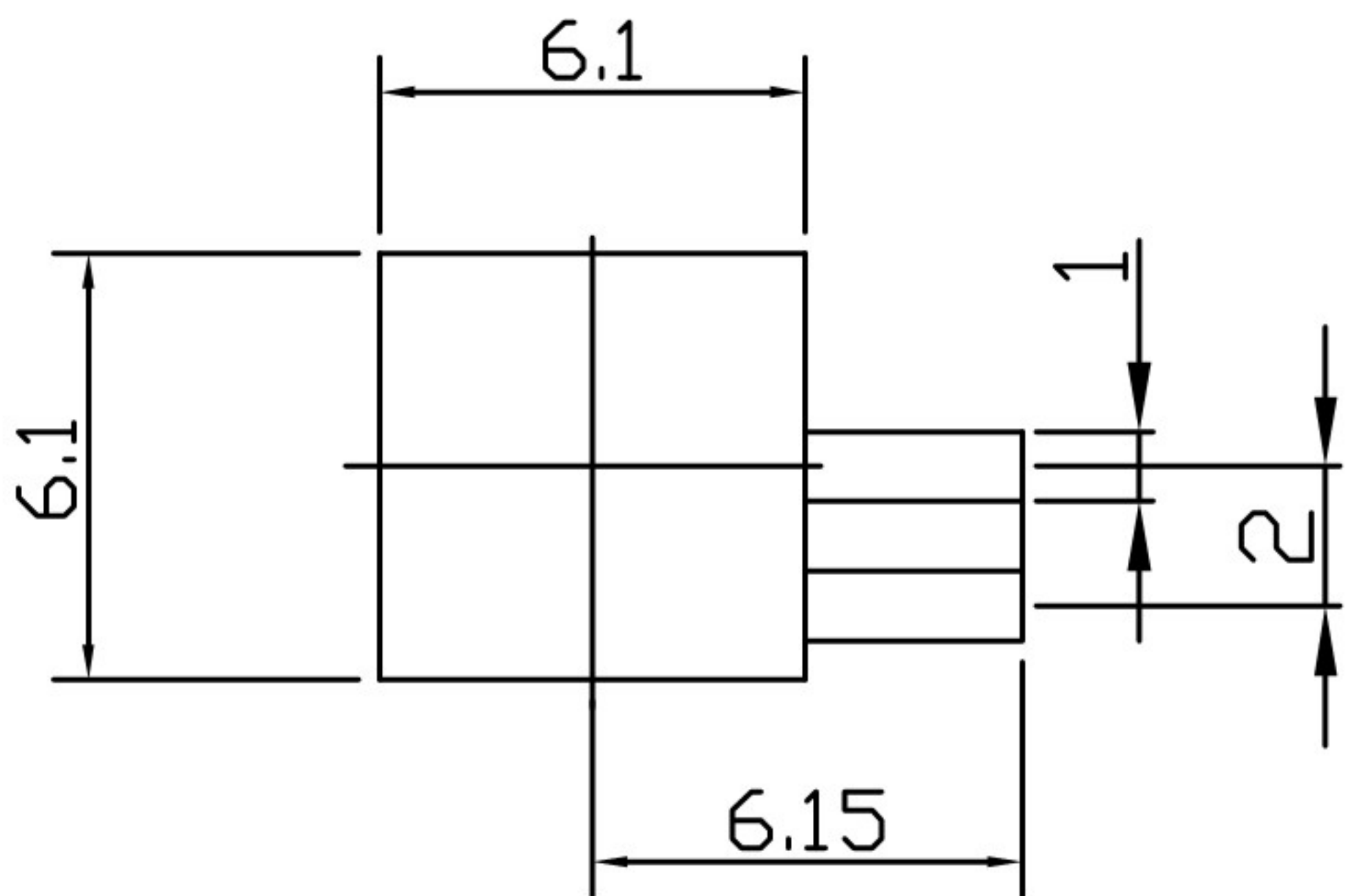
P. C. B LAYOUT
