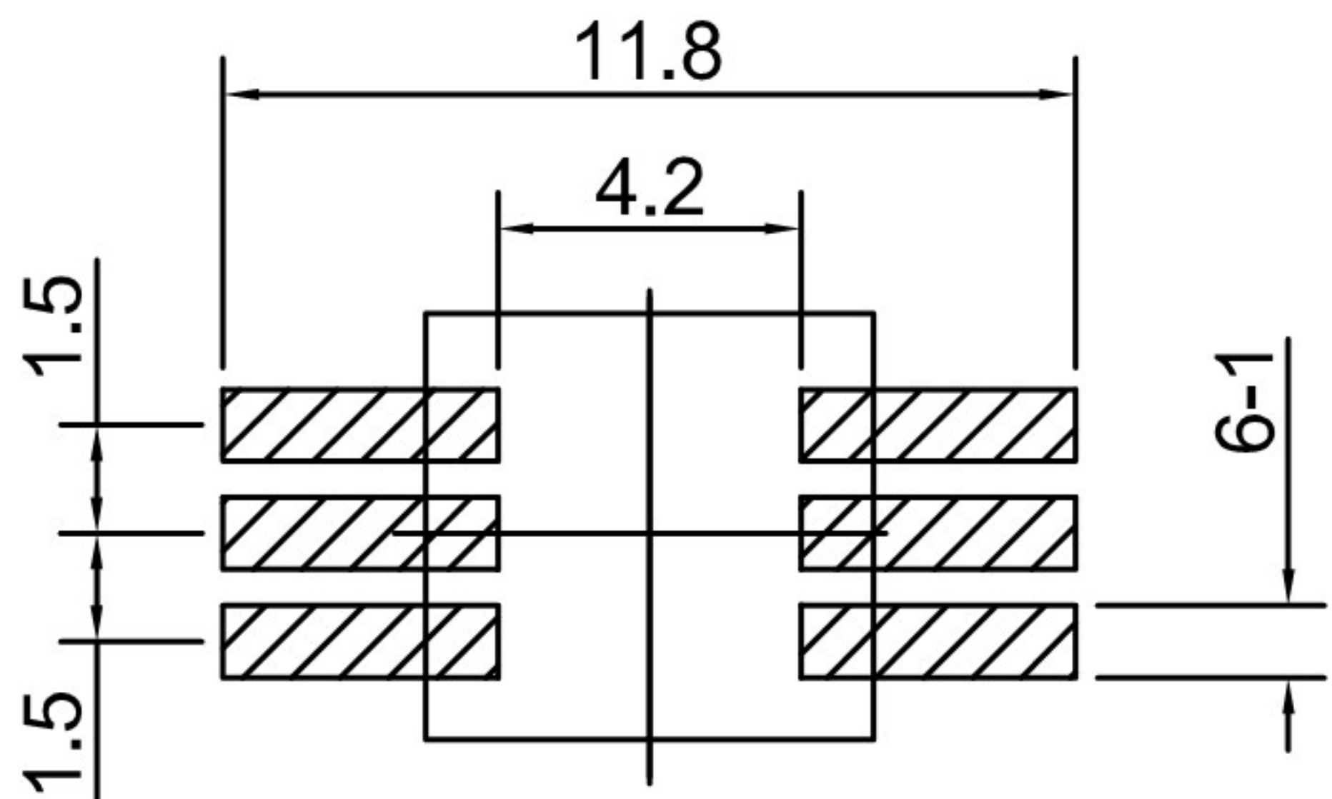
P. C. B LAYOUT
