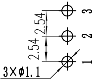
RECOMMENDED PCB LAYOUT
