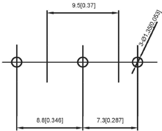
Straight PCB Terminal
