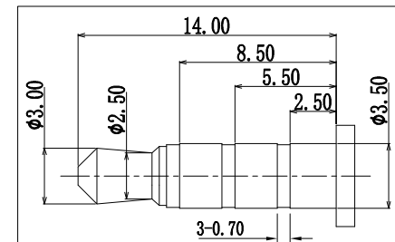
( \varnothing 3.50\text{mm} 4 POLE PLUG DETAIL DRAWING)
