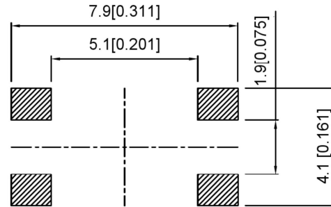
P.C.B MOUNTING PATTERN DIMENSION
