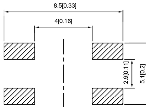
SMD REFLOW PATTERN(N/S:±0.1)
