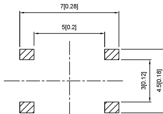
PCB LATOUT TOP VIEW
