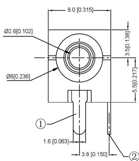
PCB
