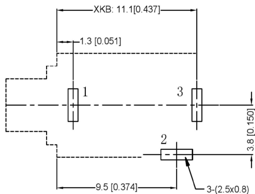
PCB
