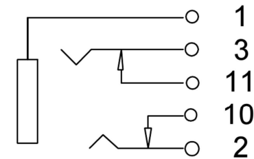
SCHEMATIC
