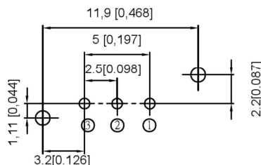
P.C.B LAYOUT MOUNTING PATTERN
