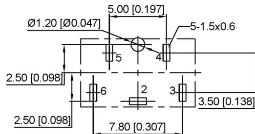
PCB HOLES(TOP VIEW) GENERAL TOLERANCE:0.1mm
