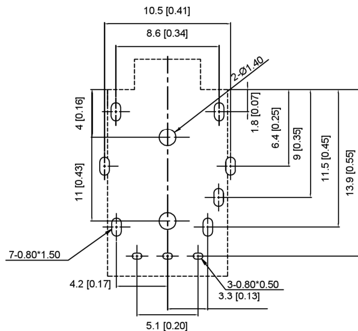
PCB LAYOUT BOTTOM VIEW TOLERANCES:±0.05
