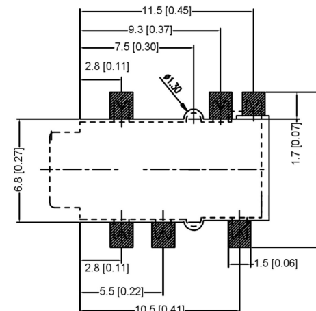
PCB LAYOUT TOP VIEW TOLERANCES:±0.05
