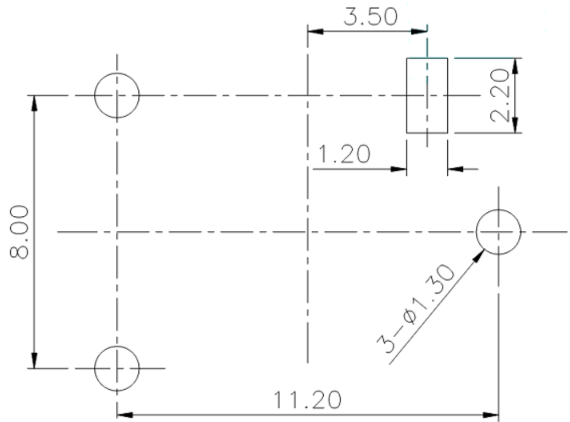
PCB LAND DIMENSION
