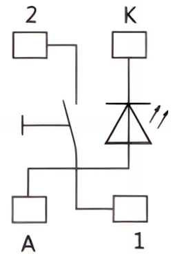
CIRCUIT
