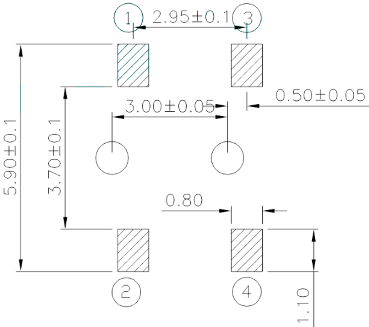
PCB LAND DIMENSION
