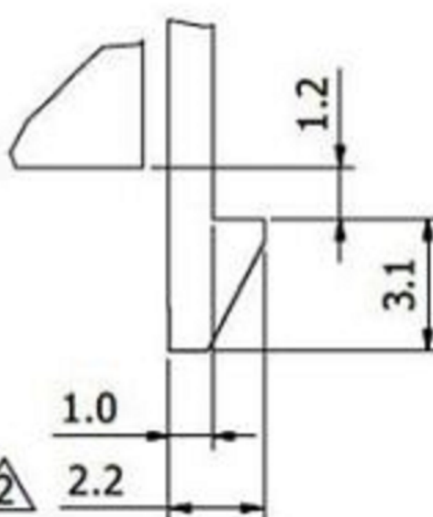
DETAIL OF "A"
