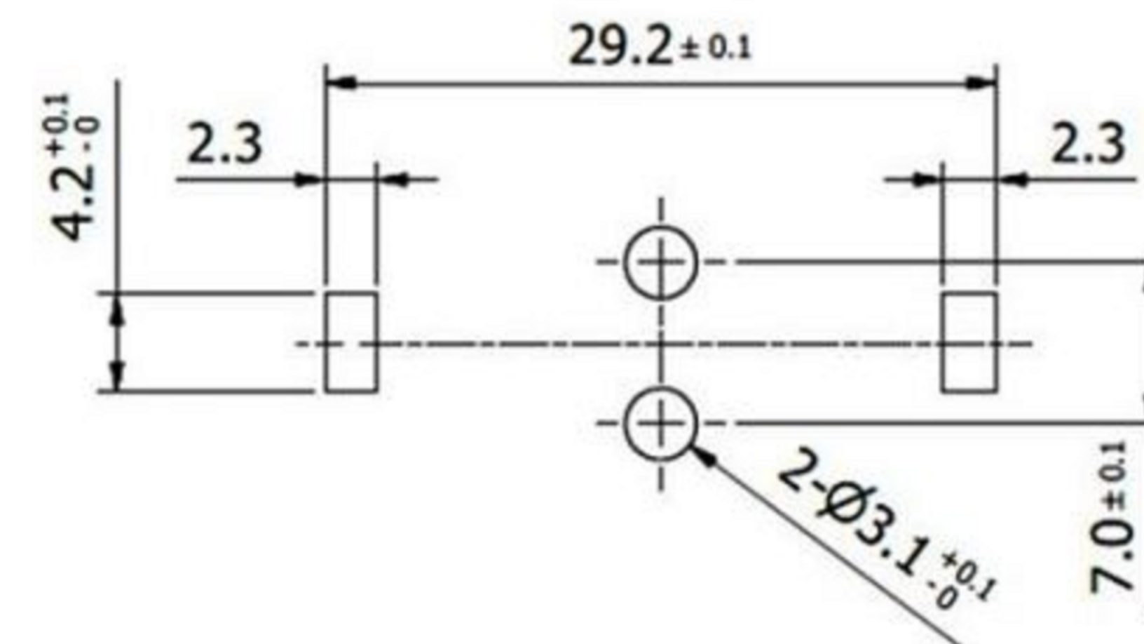
PCB MOUNTING HOLE DIMENSION
