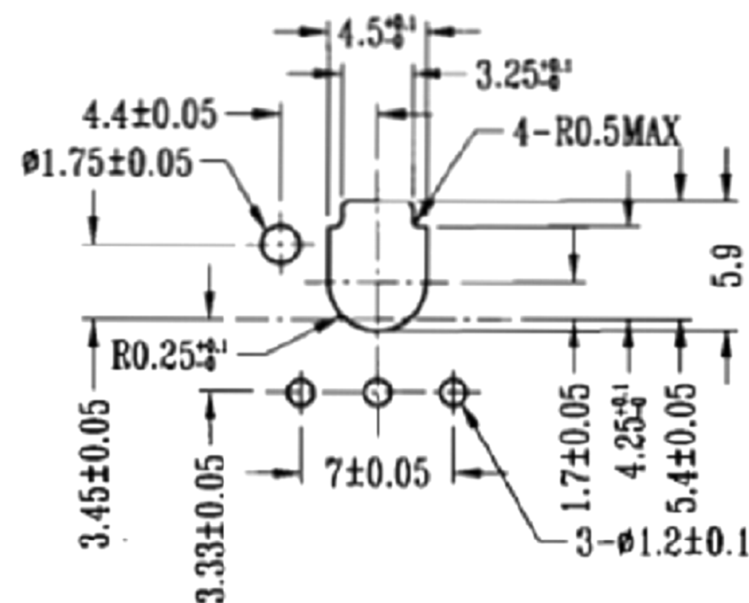
P. C. B LAYOUT
