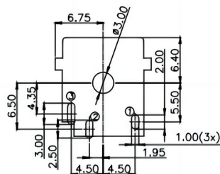
TOP VIEW (TOLRANCE:±0.05) RECOMMENDED P.C.B LAYOUT
