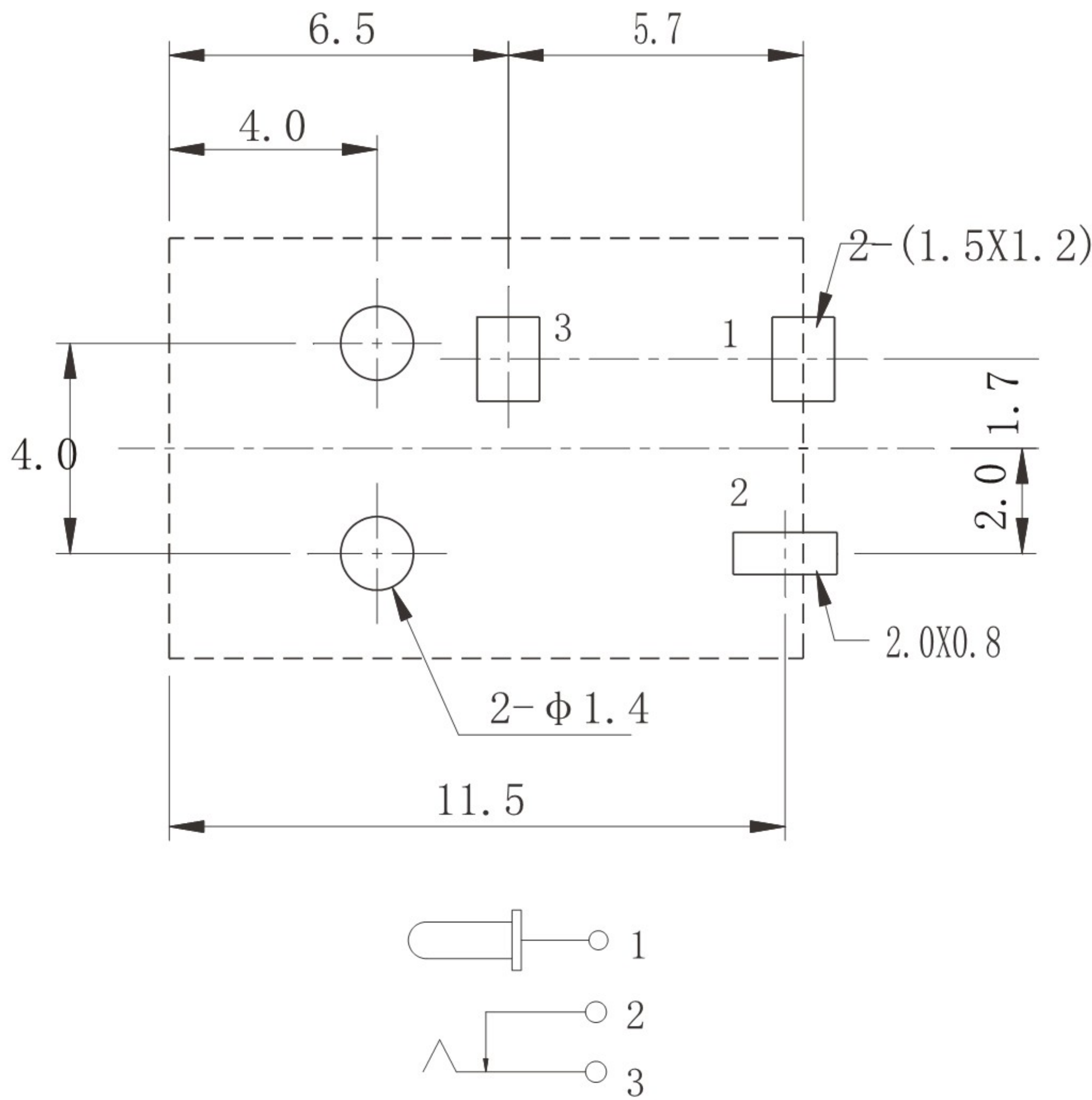
P. C. B LAYOUT TOP VIEW
