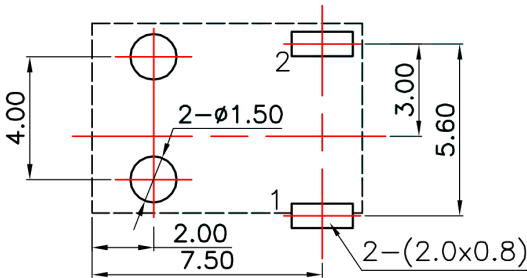
P.C.B LAYOUT(copper-sided view)
