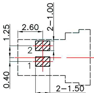
P.C.B LAYOUT(Copper-side view)
