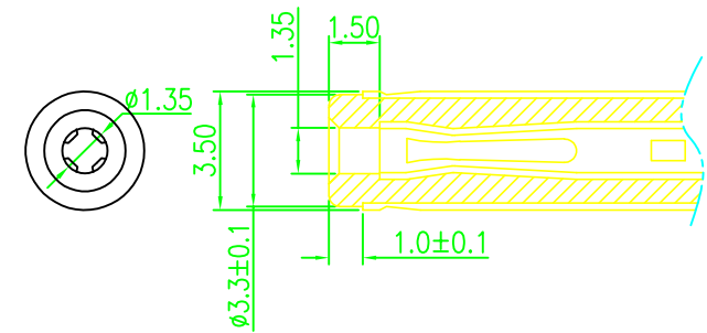
MATE PLUG
