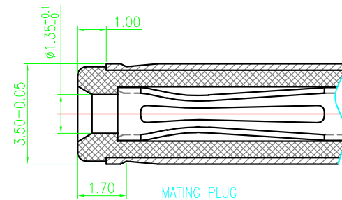
MATING PLUG P/N: DP350135-0120-60000H
