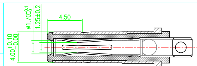
MATING PLUG DP400170-0038-60000H
