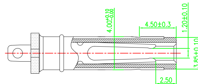
MATING PLUG P/N:DP400170-0001-60000H
