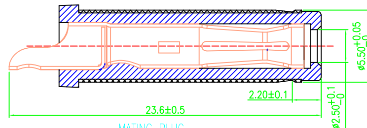
MATING PLUG P/N.: DP550250-0063-60000H
