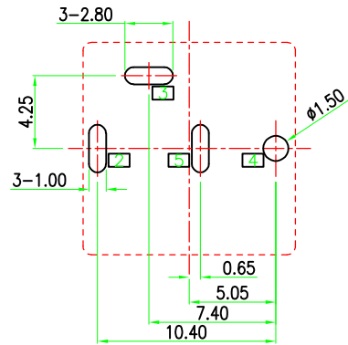
Mounting Dimension(Copper Side View) Tolerance \pm 0.1
