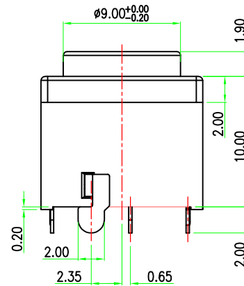
Mounting Dimension(Copper Side View) Tolerance \pm 0.1
