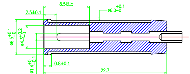
MATING PLUG P/N.: DP650140-0076-60000H
