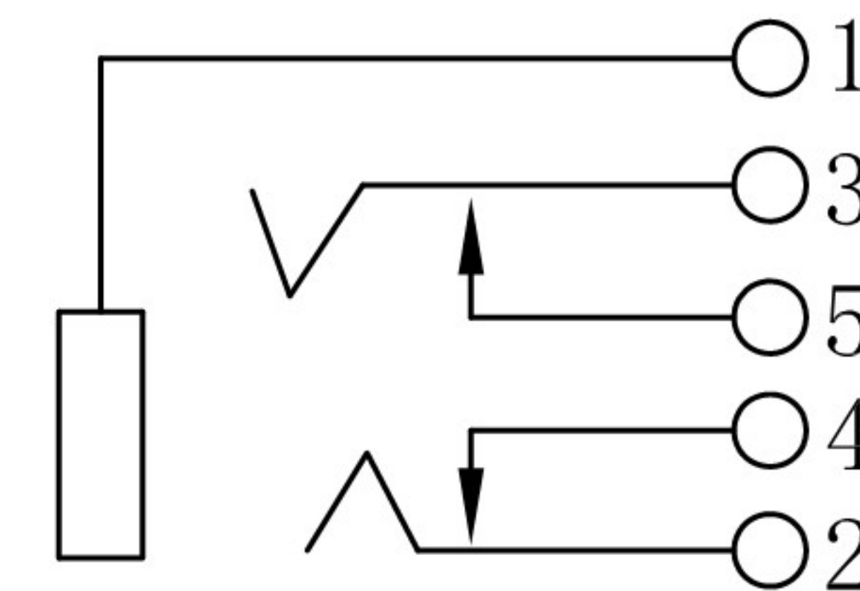
Circuit Diagram
