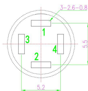
T:1.6 Dimensions of PC board holes Tolerance : \pm 0.1 (Printed-sided view)
