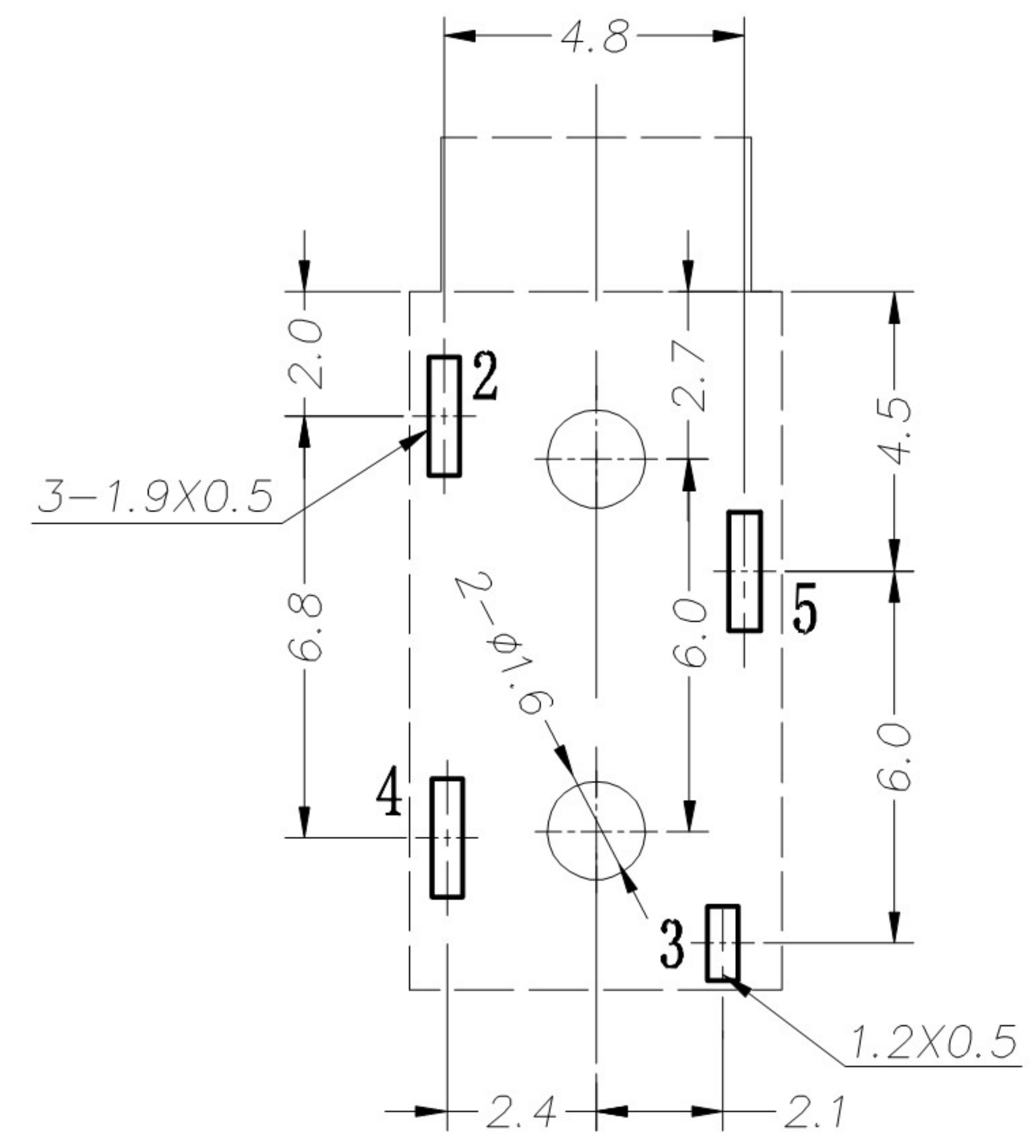
P.C.B LAYOUT TOP VIEW
