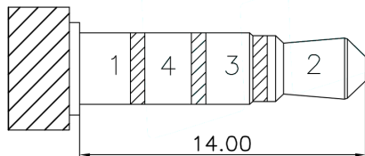
ø3.5 MATE PLUG
