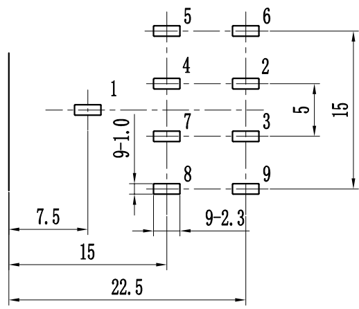
P. C. B LAYOUT (BOTTOM VIEW) Tolerance: ±0.05
