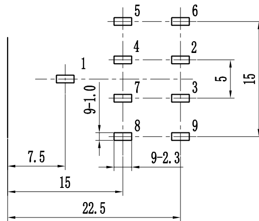
P. C. B LAYOUT (BOTTOM VIEW) Tolerance: \pm 0.05
