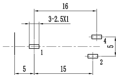
P.C.B LAYOUT (TOP VIEW) Tolerance: ±0.05
