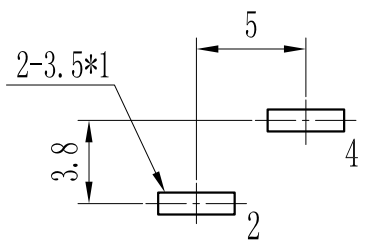
P. C. B LAYOUT (BOTTOM VIEW) Tolerance: ±0.05
