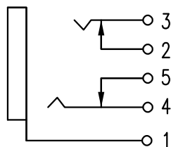
Electrical schematic
