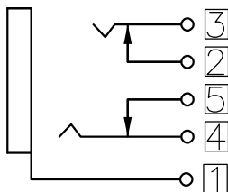
Electrical schematic
