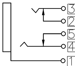
Electrical schematic
