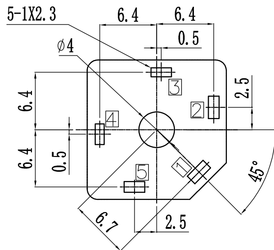
Tolerance: \pm 0.05
