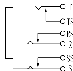
Electrical schematic
