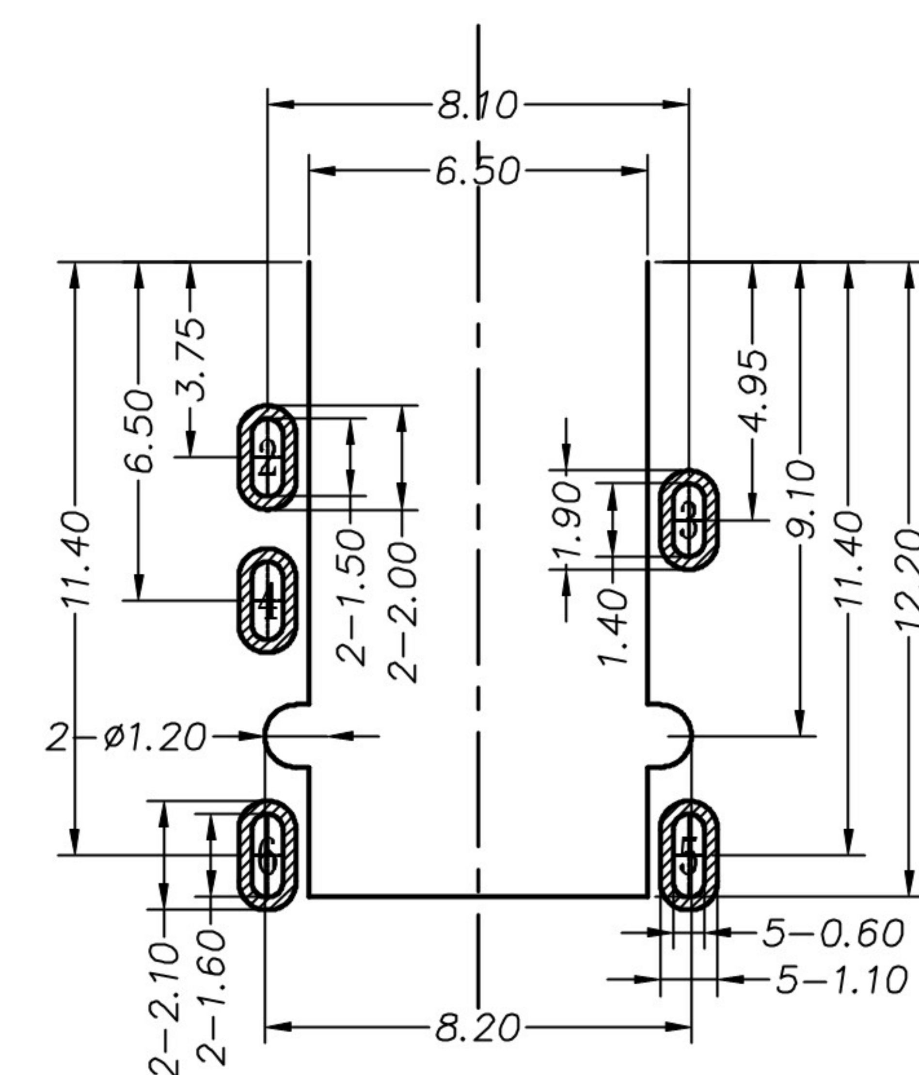
P. C. B LAYOUT TOP VIEW
