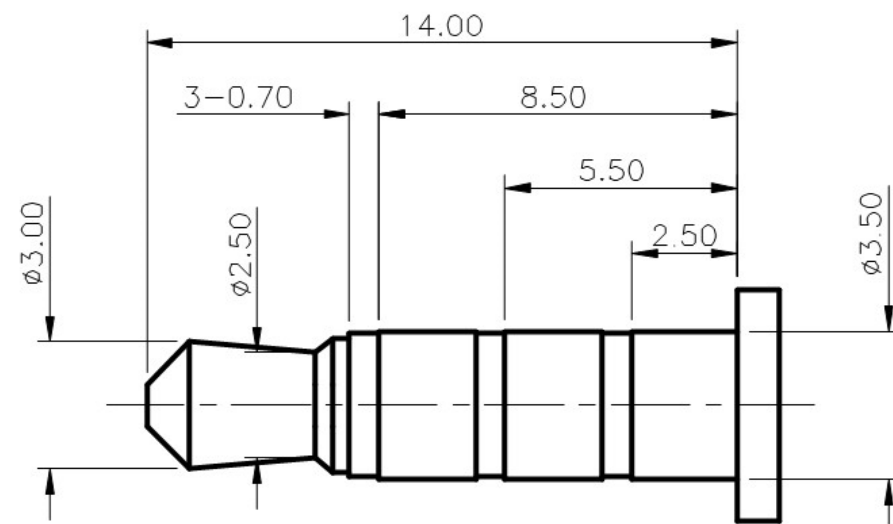
(ø3.50mm 4 POLE PLUG DETAIL DRAWING)
