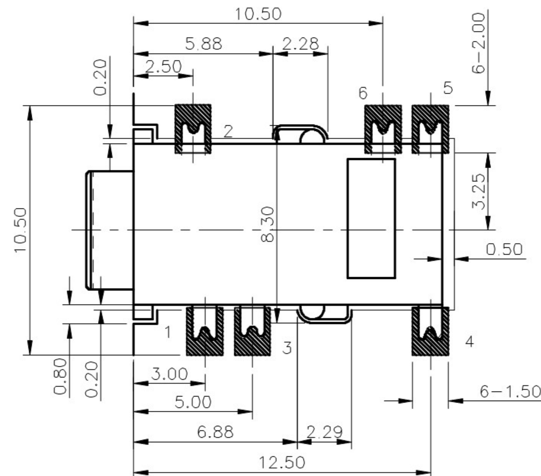
P.C.B LAYOUT TOP VIEW POSITIVE
