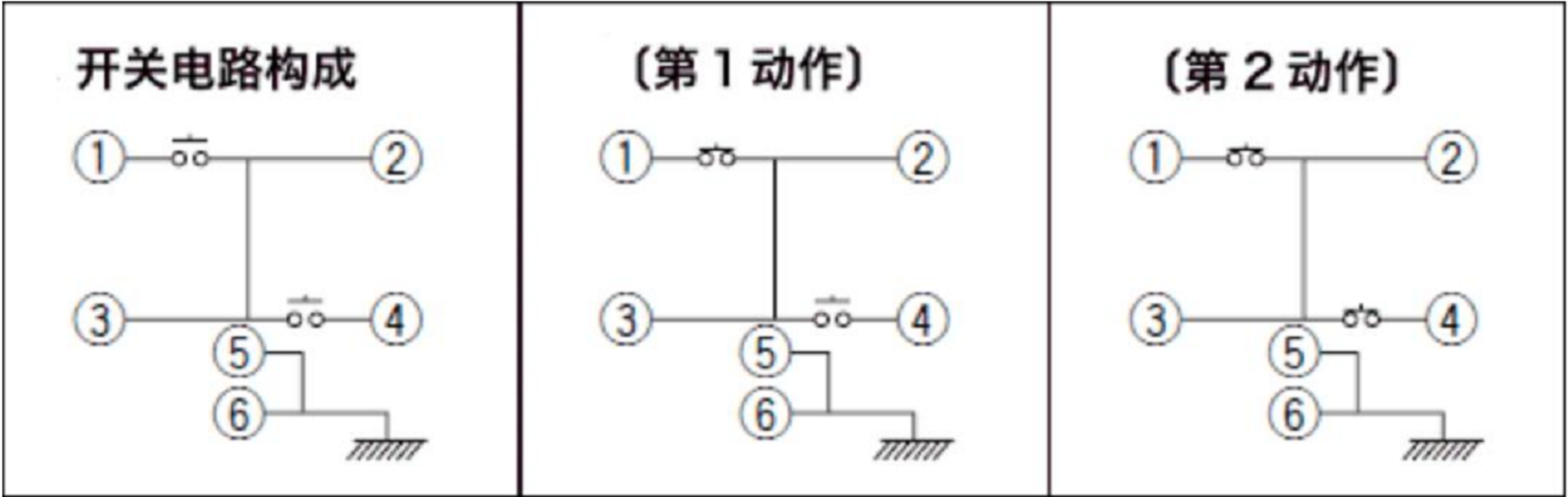
SCHEMATIC
