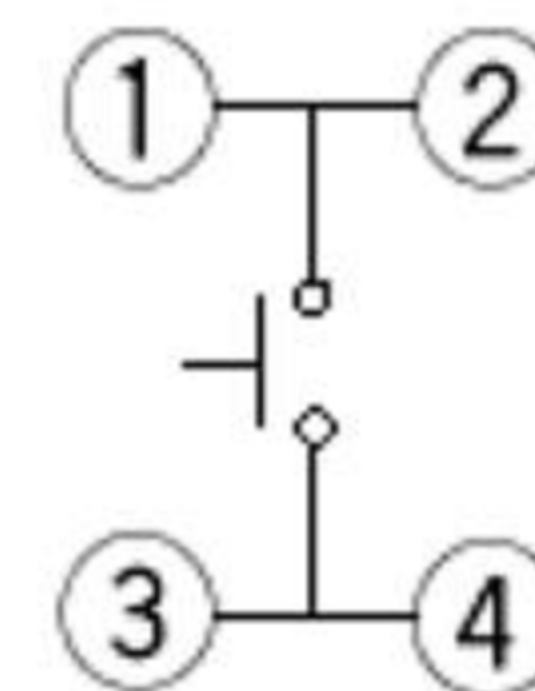
SCHEMATIC
