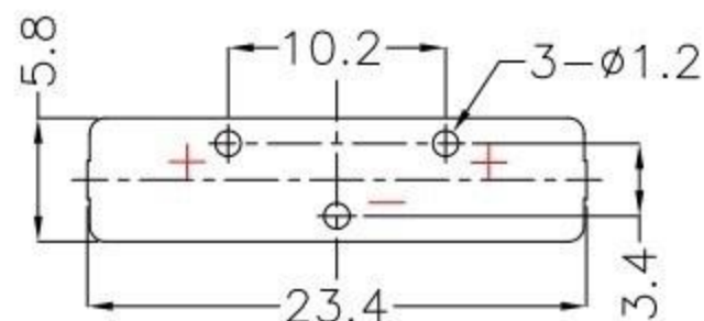
PCB Layout Diagram Top View
