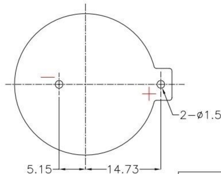
PCB Layout Diagram Top View
